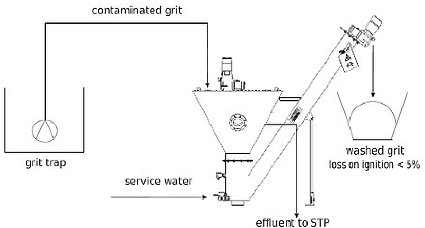
Process diagram
