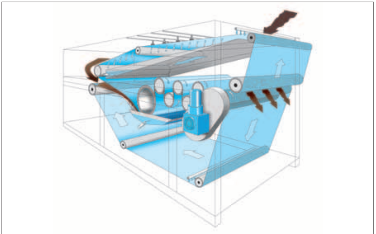
HUBER Bogenpress BS with 8 rolls
